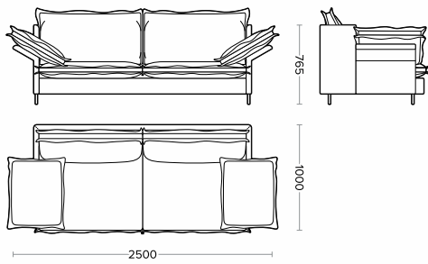
GRAND/2P/2A/2500/1000
