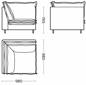
GRAND/C/980/980
