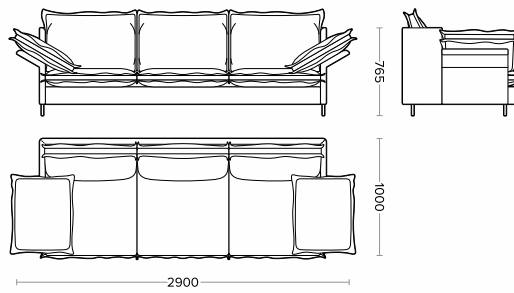
GRAND/3P/2A/2900/1000
